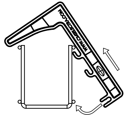
Alternative Brackets
